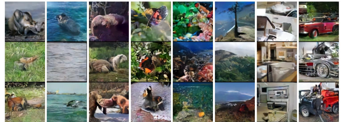
Figure 3: Samples (128x128) from a VQ-VAE with a PixelCNN prior trained on ImageNet images. From left to right: kit fox, gray whale, brown bear, admiral (butterfly), coral reef, alp, microwave, pickup.
