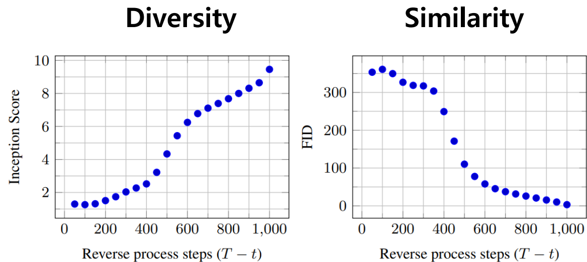
Figure 10: Unconditional CIFAR10 progressive sampling quality over time
